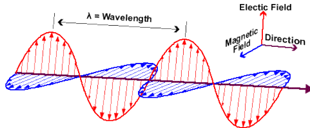
Figure 31: An electromagnetic wave consists of oscillating electric and magnetic fields, which are perpendicular to each other and also perpendicular to the direction of motion of the wave.
