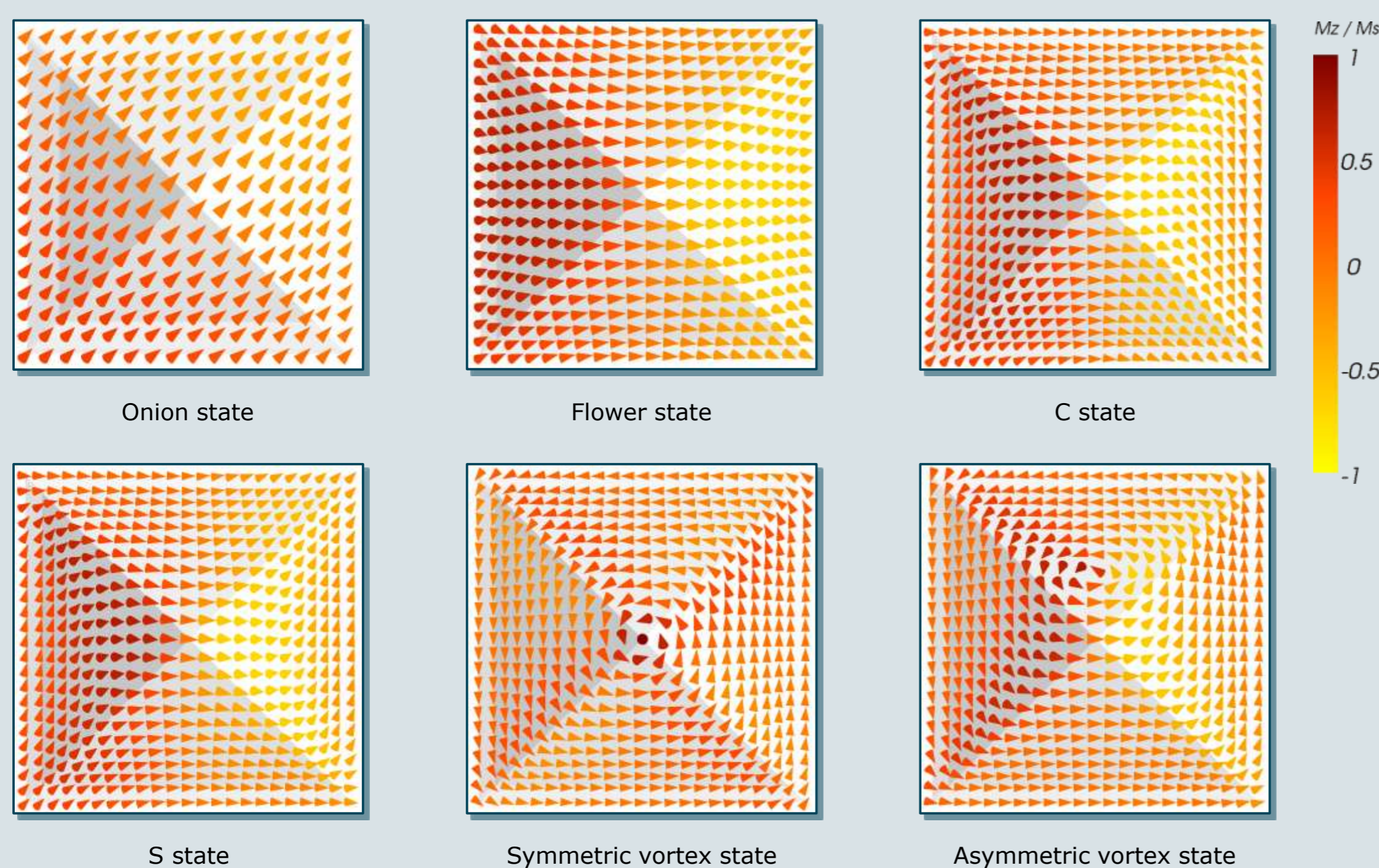
Figure 4: Illustration of observed micromagnetic configurations. The pyramidal structures are viewed from the top (the z direction of figure 3). The z component of the (normalised) magnetisation is denoted by the color bar. The names of the states derive from their appearance, e.g. the C state has its name as it resembles the letter C rotated 90 degrees clock wise. Only the S state is no micromagnetic ground state.
