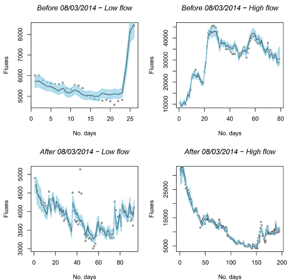
Fig. 10. Nitrate fluxes ( \text{kg/day} ) for the entire study period using the estimated parameters for the change-point structures. Black dots are the observed fluxes, black solid line represents the fluxes estimated from model M1 and shaded area represents the 95% CI for the estimated fluxes.
