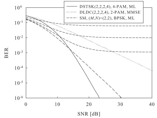
Fig. 5. Achievable BER curve of our DSTSK scheme, compared with the DLDC scheme as well as the SM scheme suffering from the CSI estimation error.
