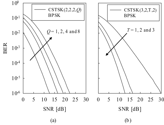
Fig. 3. Achievable BER curves of our CSTSK system, comparing the effects of (a) the number of dispersion matrices Q and (b) the space-time block duration T .
