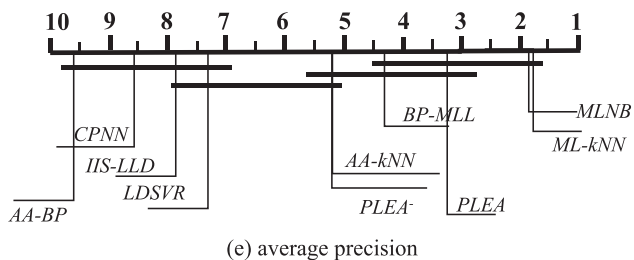
Fig. 12. CD diagrams given CD = 2.7053 of Nemenyi tests on the 10 algorithms for average precision evaluation metric.
