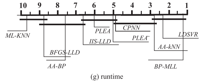
Fig. 7. CD diagrams given CD = 2.1613 of Nemenyi tests on the 10 algorithms and 15 datasets for run time (s) evaluation metric
