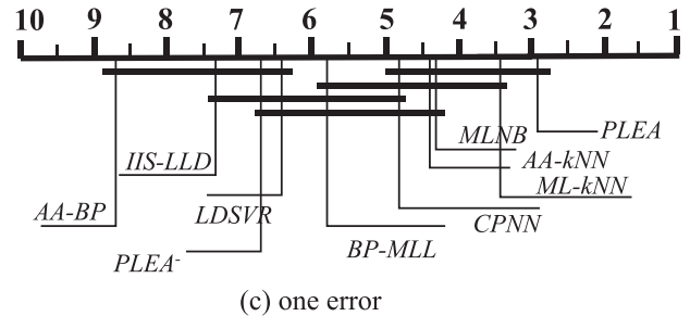
Fig. 10. CD diagrams given CD = 2.7053 of Nemenyi tests on the 10 algorithms for one error evaluation metric.
