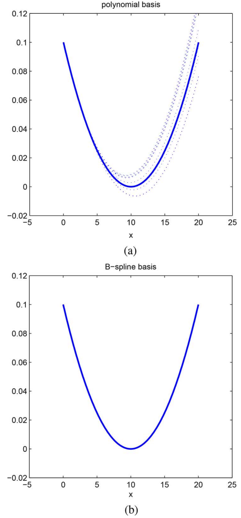
Fig. 2. Illustration of the superior numerical stability of the B-spline model over the polynomial model. (a) Polynomial basis and (b) B-spline basis.
