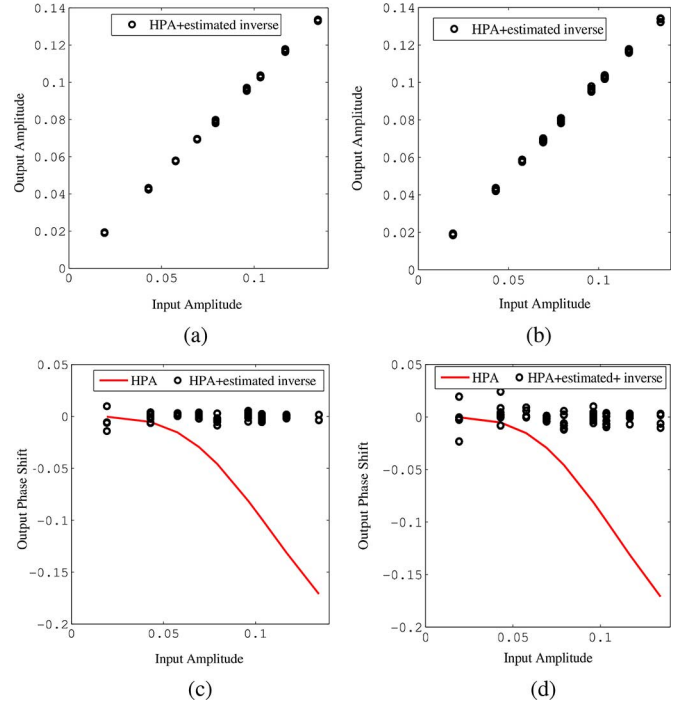
Fig. 4. Combined response of the true HPA and its estimated inversion obtained under OBO = 3 dB and E_b/N_o = 4 dB: (a) combined amplitude response by Scheme 1; (b) combined amplitude response by Scheme 2; (c) combined phase response by Scheme 1; and (d) combined phase response by Scheme 2.
