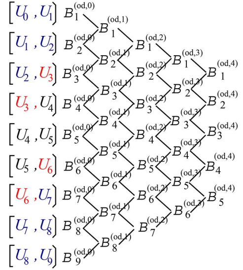
Fig. 1. Visualization of the De Boor recursion for P_o = 4 and N_{od} = 5 , where U_{\min} = U_3 and U_{\max} = U_6 .
