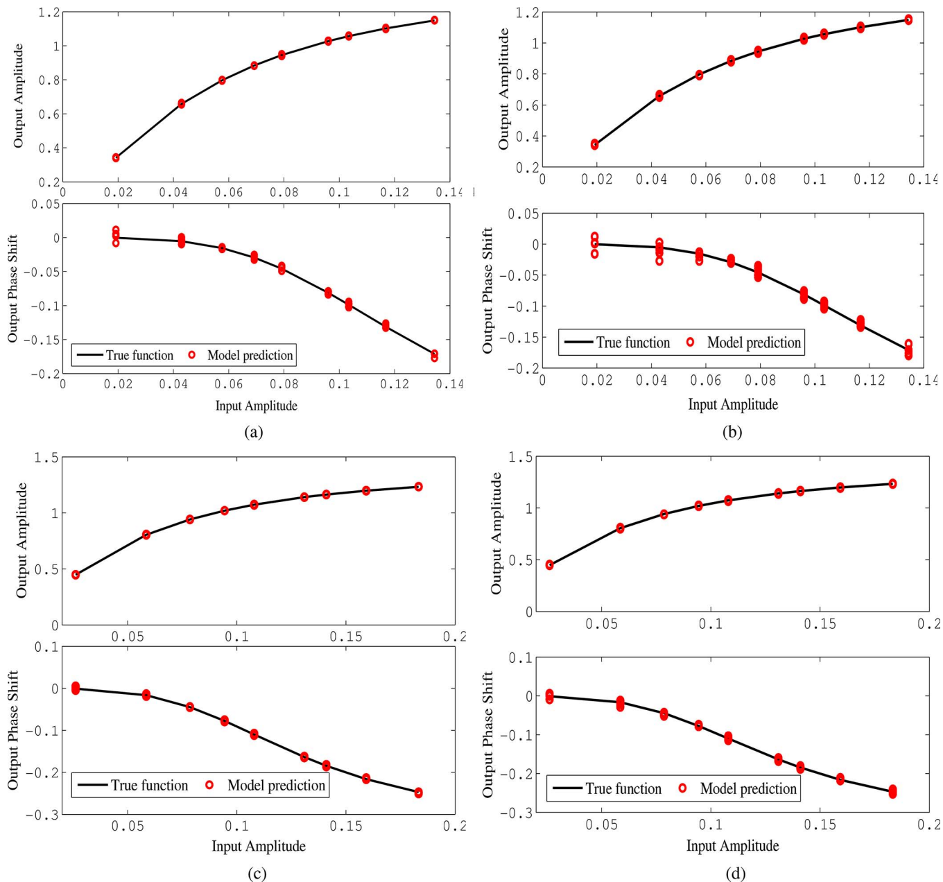
Fig. 3. Comparison of the HPA's nonlinearity \Psi(\cdot) and the estimated nonlinearity \hat{\Psi}(\cdot) : (a) Scheme 1 under OBO = 3 dB, E_b/N_o = 4 dB; (b) Scheme 2 under OBO = 3 dB, E_b/N_o = 4 dB; (c) Scheme 1 under OBO = 2 dB, E_b/N_o = 10 dB; and (d) Scheme 2 under OBO = 2 dB, E_b/N_o = 10 dB.
