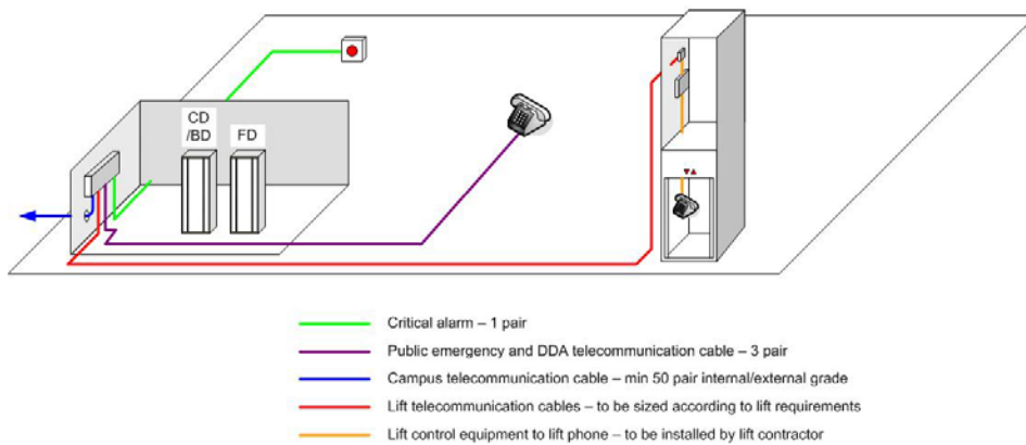
Figure 71 Voice block wiring design
