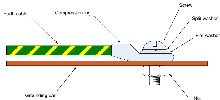
Figure 39 Detail for bonding earth cable with screw and bolt
