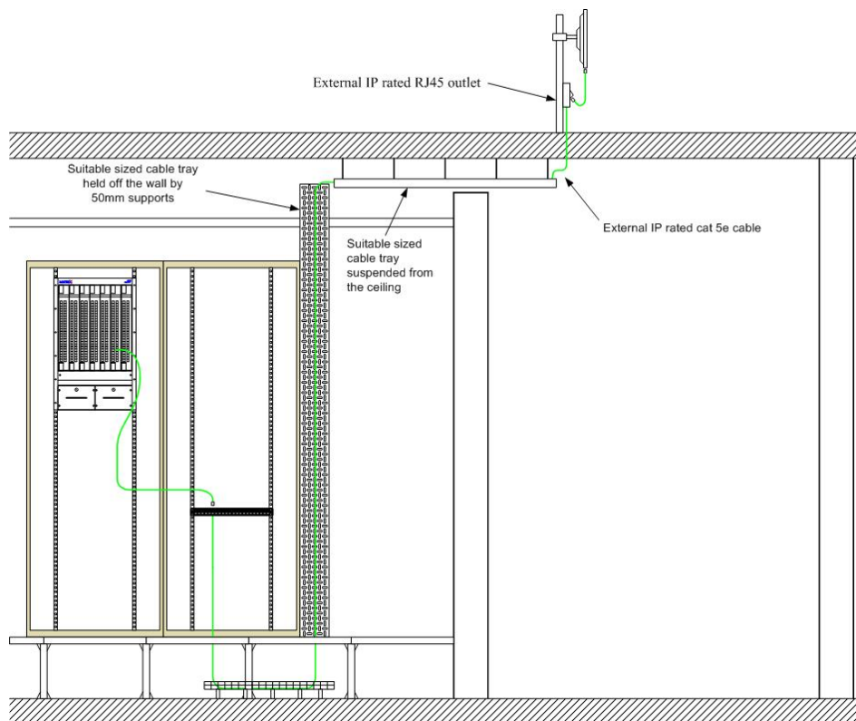
Figure 56 External mounted outlets
