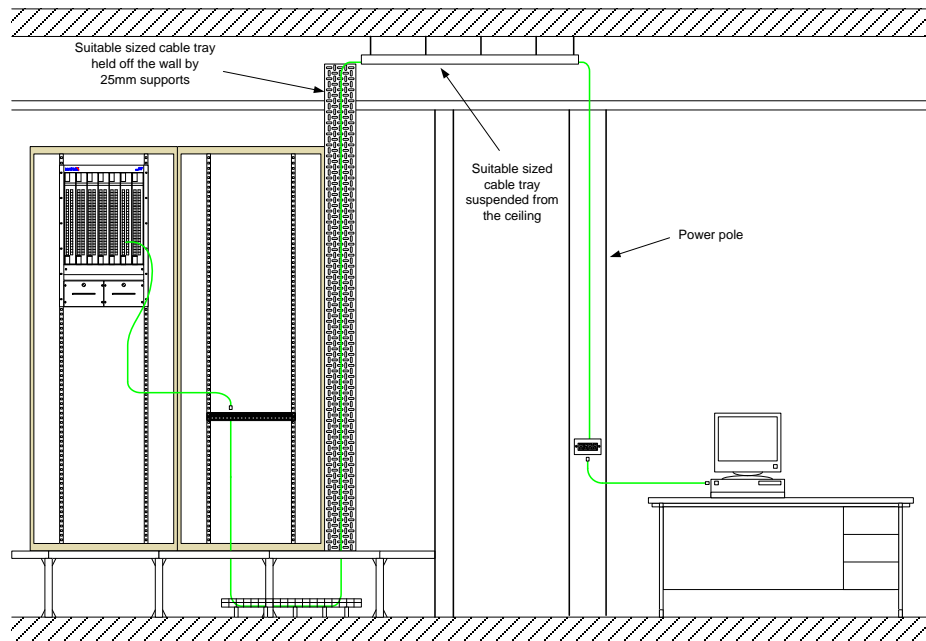
Figure 48 Power pole with consolidation point
