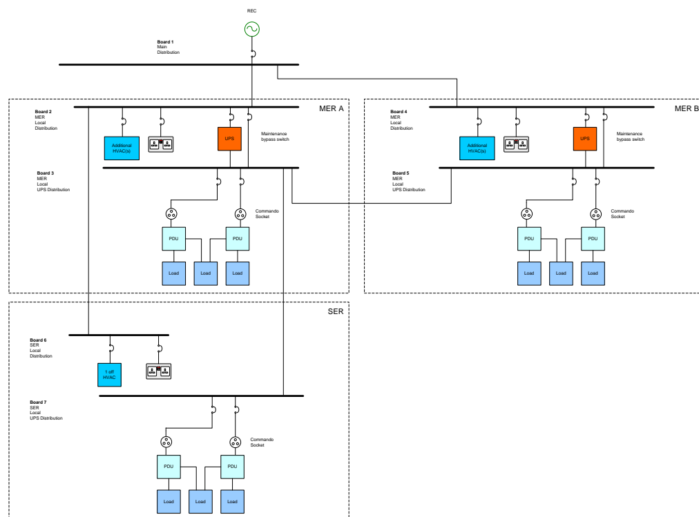
Figure 26 Typical N redundant UPS system
