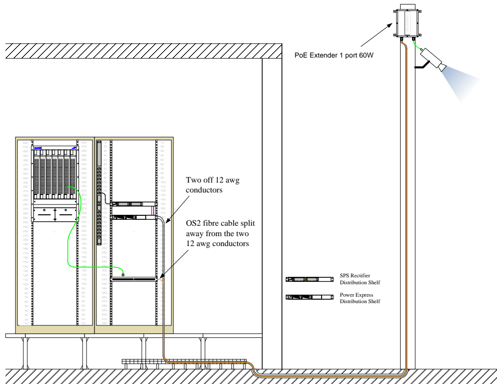
Figure 58 Powered fibre cable
