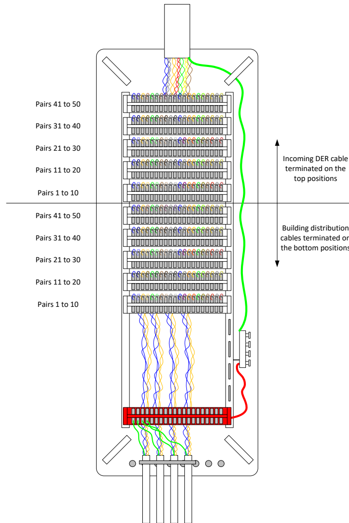
Figure 73 Telco DP box showing jumpered cross connect
