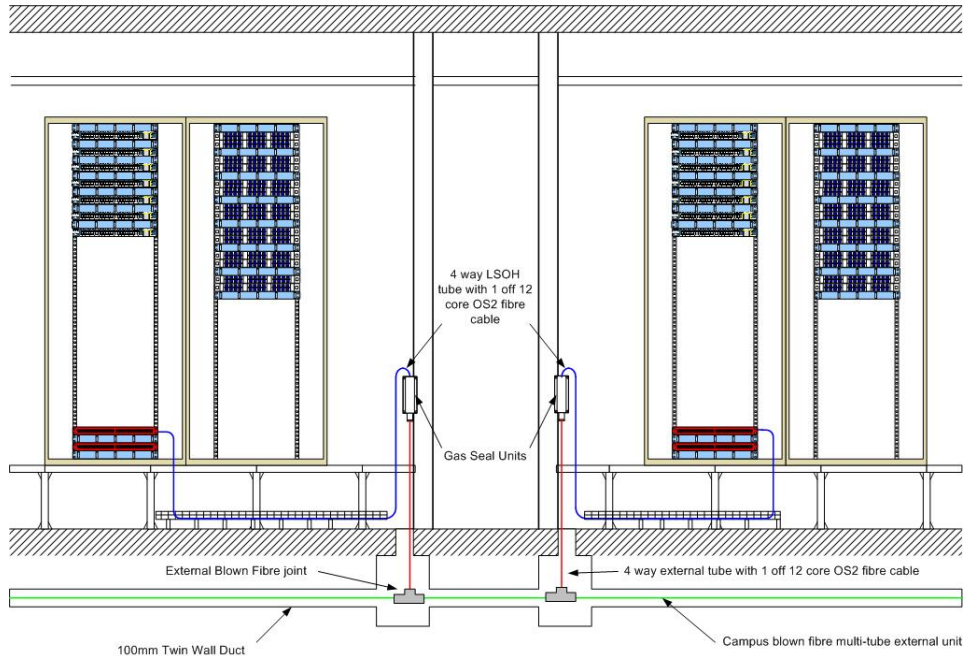
Figure 66 Campus distribution for a double MER
