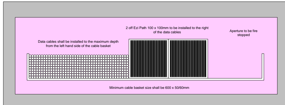
Figure 32 Cable penetration
