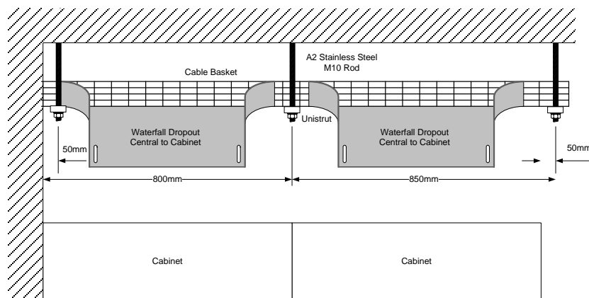
Figure 29 High level containment within a suspended ceiling side elevation
