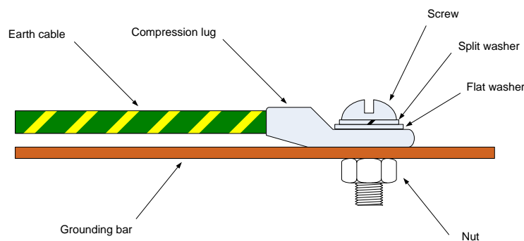
Figure 42 Detail for bonding earth cable with screw and bolt
