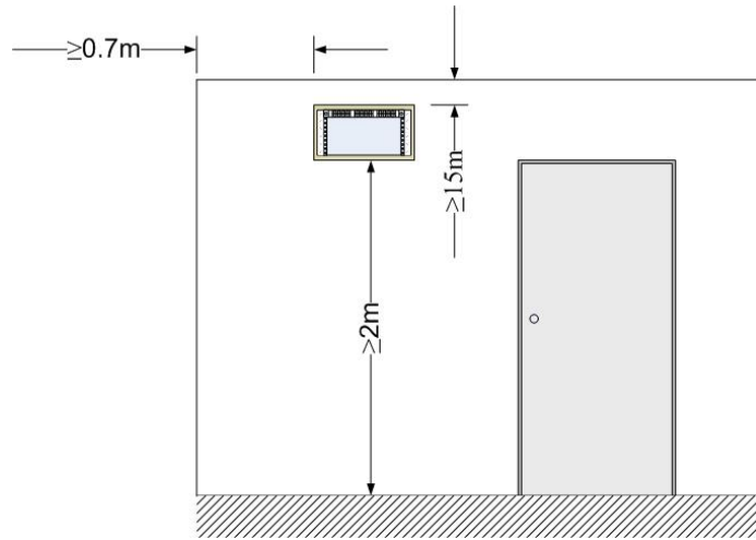
Figure 6 Desirable wall mounted box and cabinet clearances
