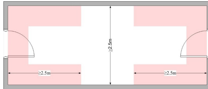
Figure 8 None designated throughway clearances for wall mounted cabinets
