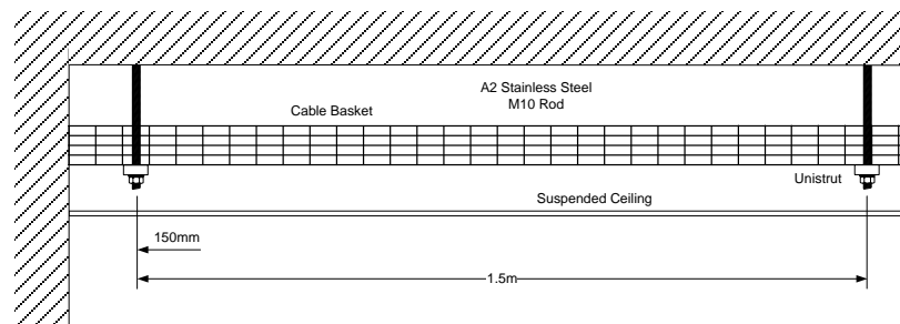
Figure 62 Suspended ceiling cable basket side elevation
