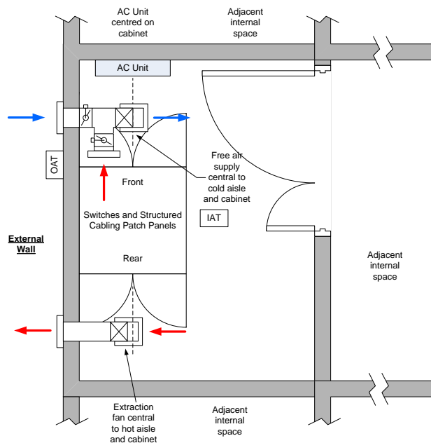
Figure 20 Example layout for a single external wall
