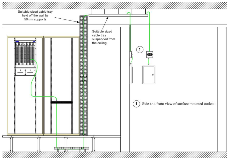
Figure 54 Surface mounted outlets
