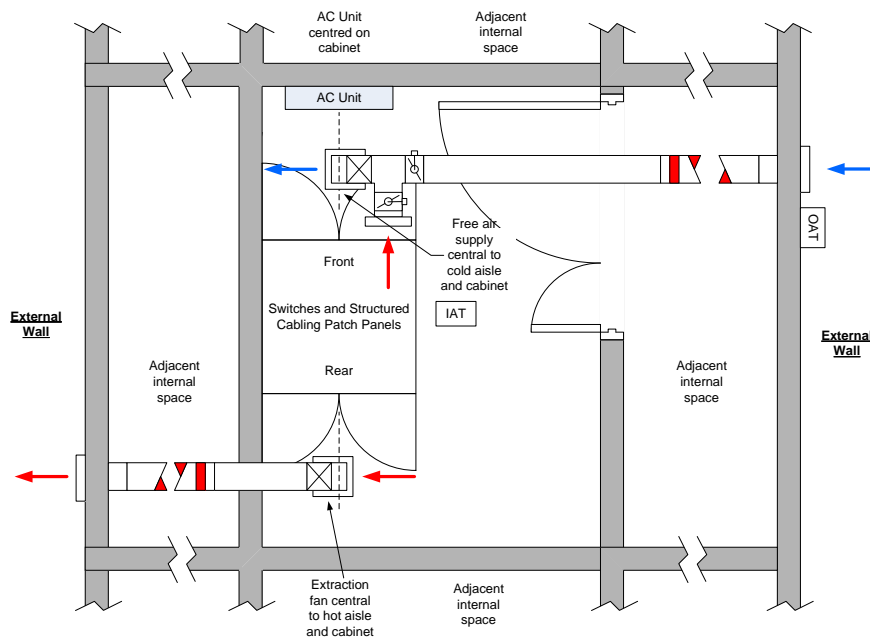
Figure 22 Example layout for 2 adjacent external walls
