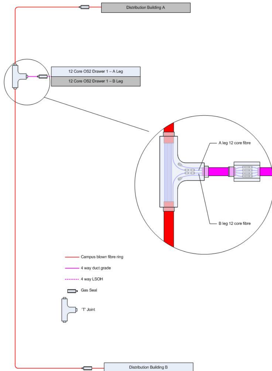
Figure 69 Single blown fibre joint arrangement
