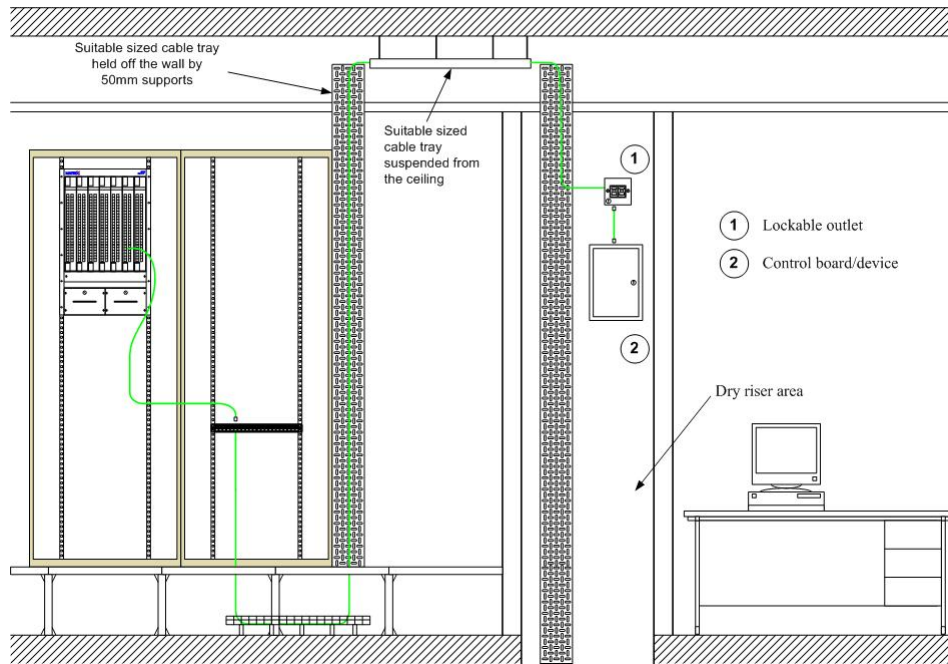
Figure 51 Dry Riser Outlets
