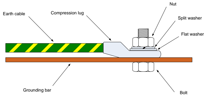
Figure 41 Detail for bonding earth cable with nut and bolt
