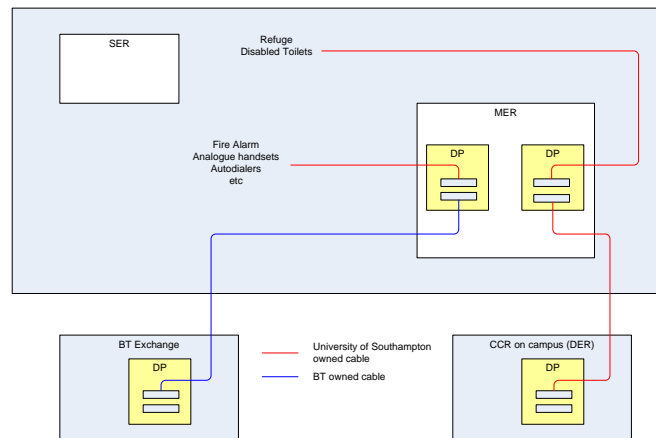
Figure 70 University and BT demarcation for voice cabling
