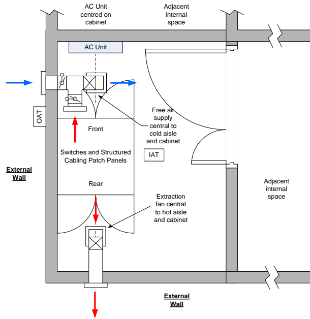
Figure 21 Example layout for a 2 adjoining external walls
