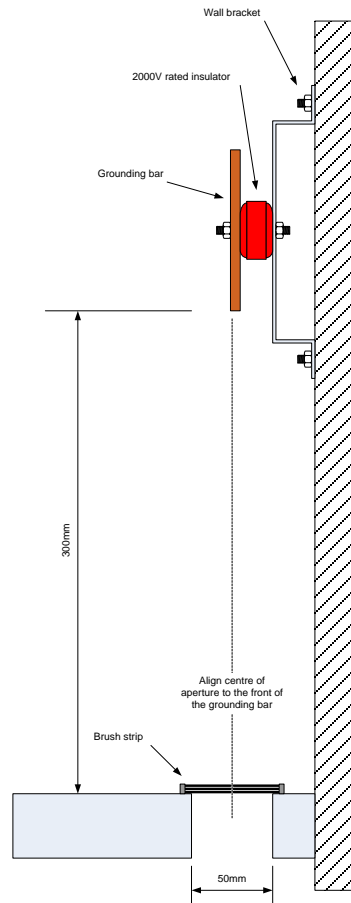
Figure 36 Grounding bar side elevation detail
