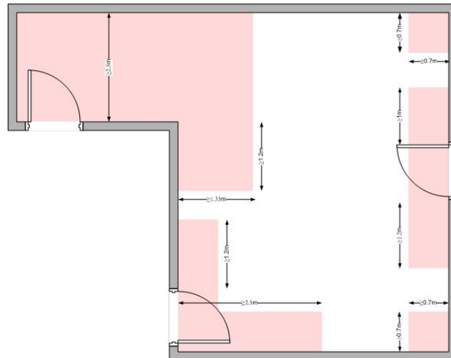
Figure 7 Single room clearances for wall mounted cabinets
