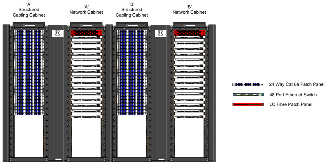
Figure 13 MER A cabinet layout
