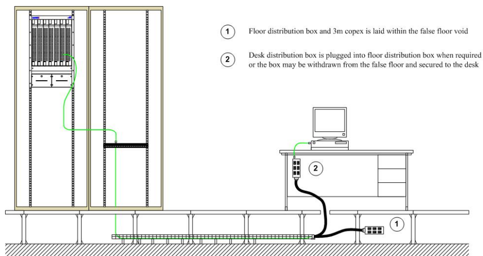
Figure 47 Under floor Minipod
