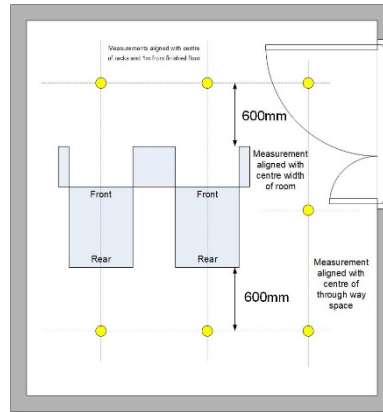
Figure 16 Lighting measurements for MER B and SERs
