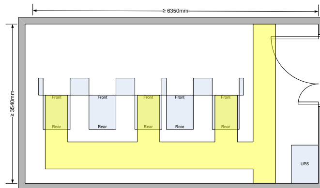
Figure 31 Suspended floor containment for MER A
