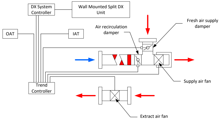
Figure 19 Logical diagram for cooling system
