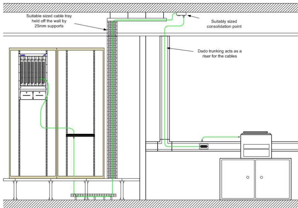
Figure 55 Temporary outlet with consolidation point
