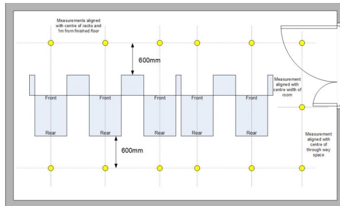
Figure 17 Lighting measurements for MER A
