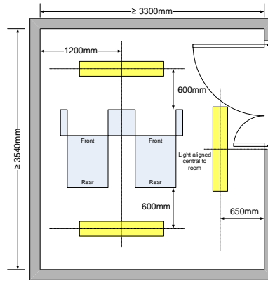
Figure 14 Lighting layout for MER B and SERs
