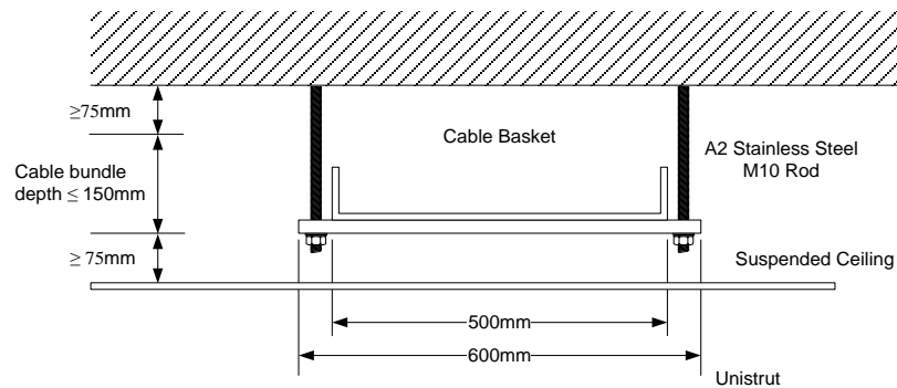
Figure 61 Suspended ceiling cable basket
