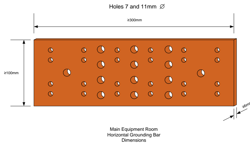
Figure 33 MER grounding bar
