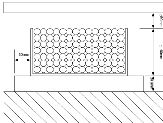
Figure 60 Suspended floor cable basket
