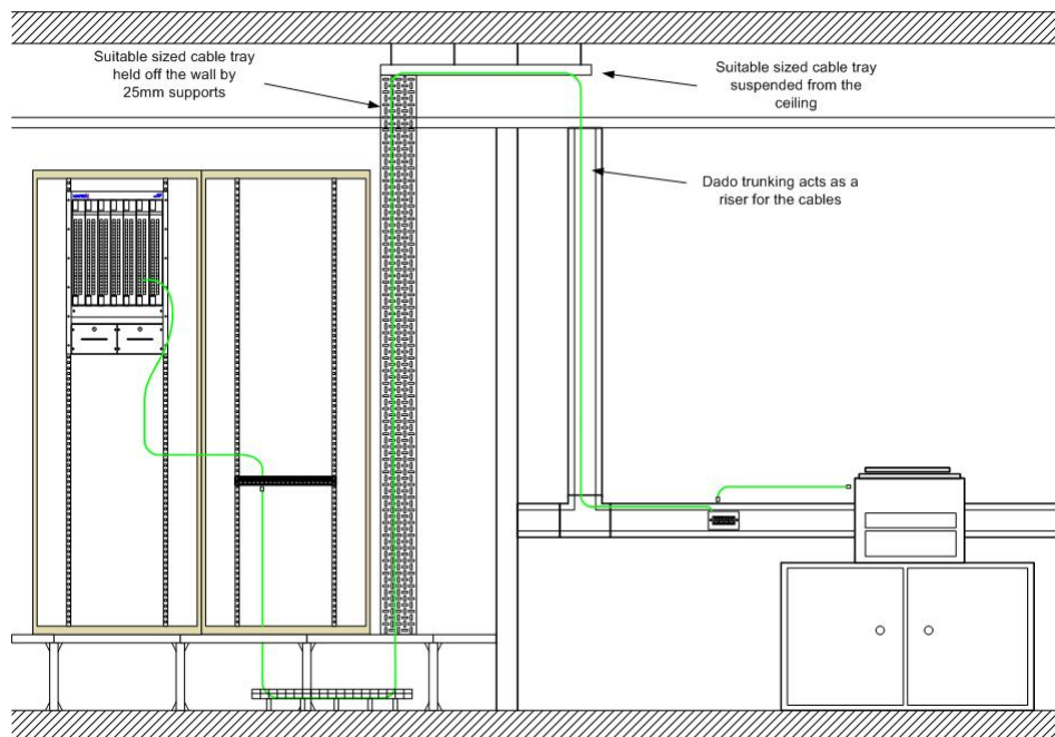
Figure 49 Dado trunking outlets
