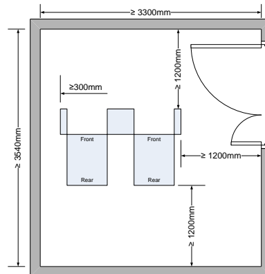
Figure 4 Telecom room layout for MER B and SERs
