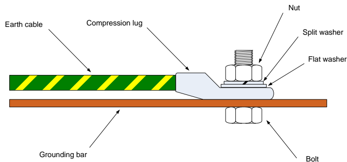
Figure 38 Detail for bonding earth cable with nut and bolt
