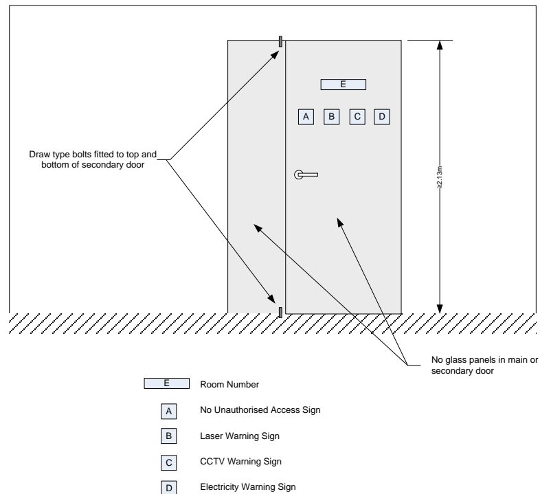
Figure 9 Telecom room door entry details
