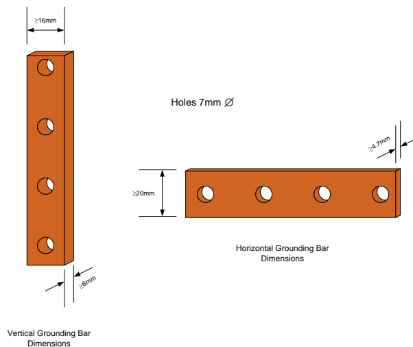
Figure 37 Cabinet grounding bar
