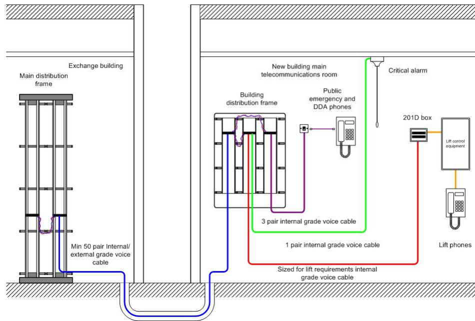
Figure 72 Building distribution backbone
