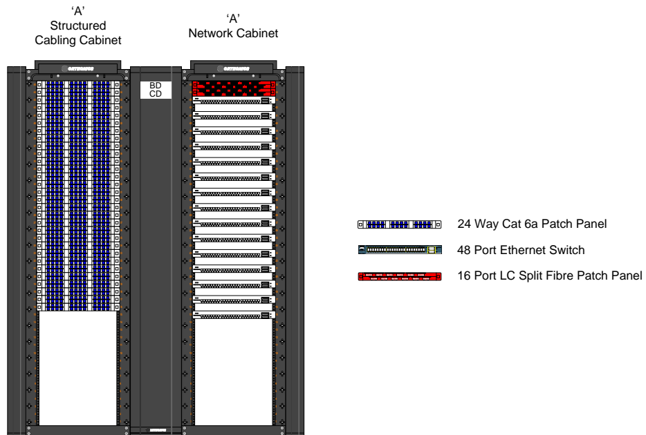
Figure 12 MER B cabinet layout
