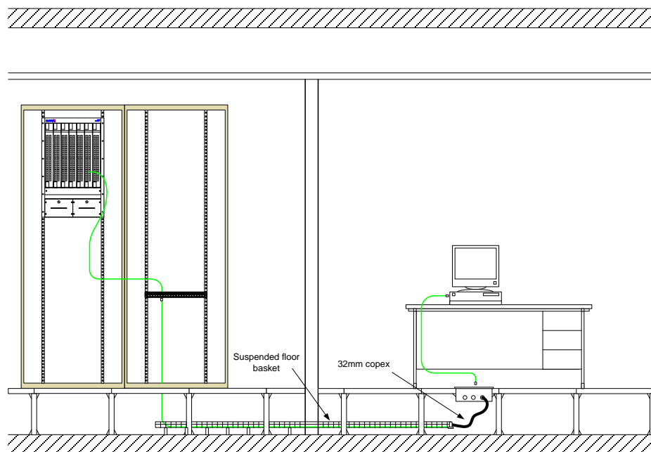
Figure 45 Floor box
