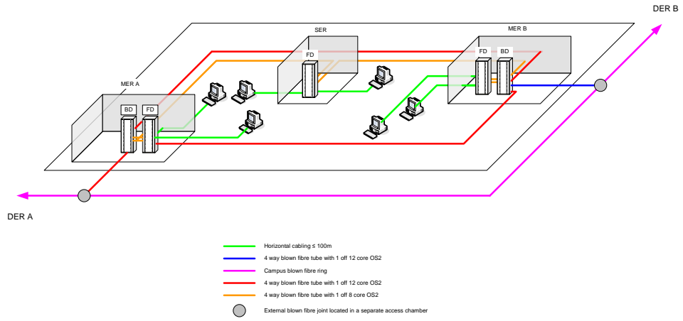
Figure 65 Double MER blown fibre
