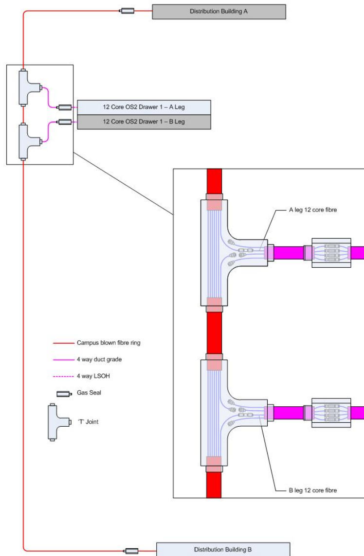
Figure 68 Dual blown fibre joint arrangement
