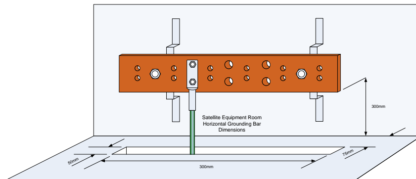
Figure 35 Grounding bar front elevation detail
