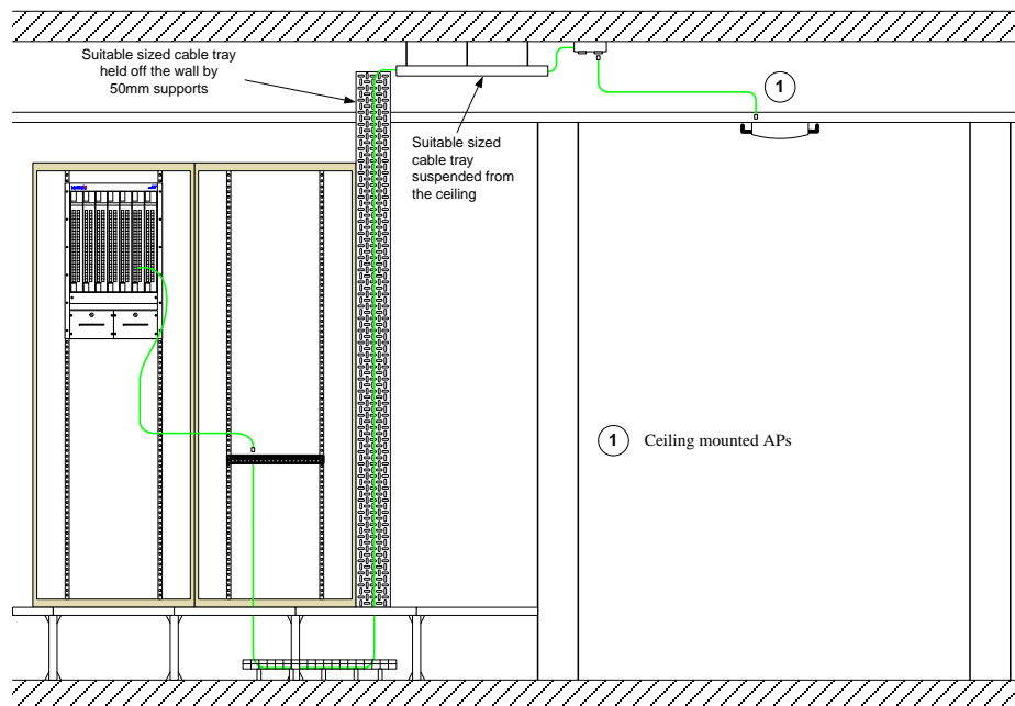
Figure 52 Suspended ceiling outlets
