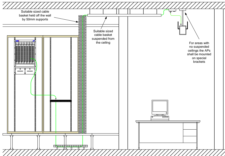
Figure 53 Ceiling mounted with no suspended ceiling outlets
