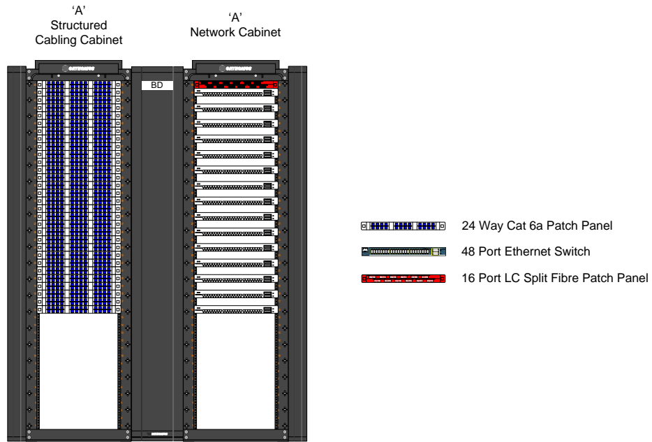
Figure 11 SER cabinet layout
