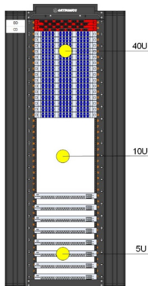
Figure 18 Front view of cabinet lighting test points
