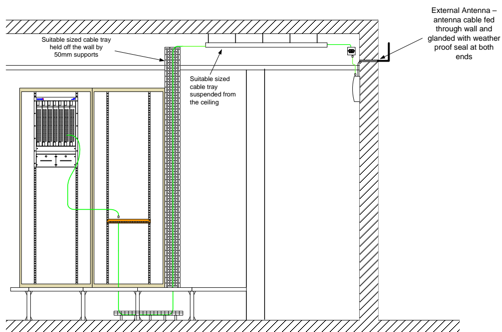
Figure 57 External mounted wireless APs
