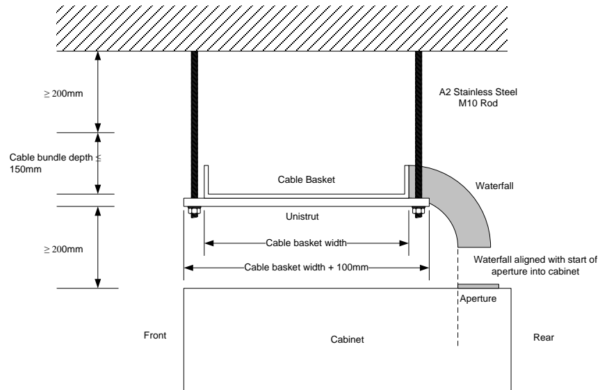
Figure 28 High level containment with no suspended ceiling
