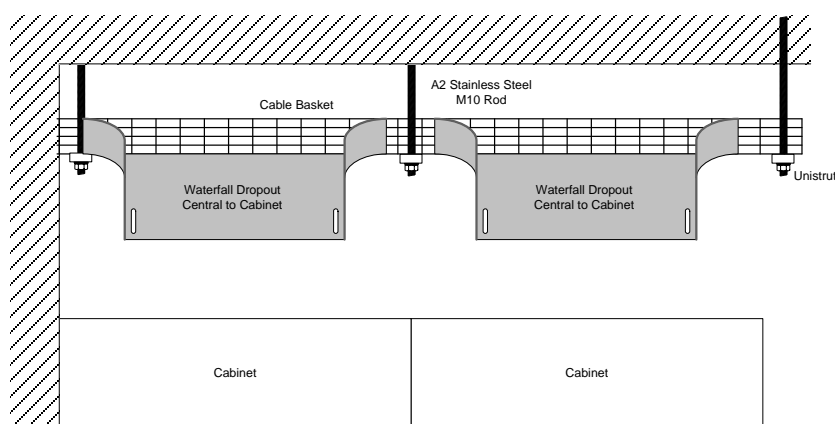
Figure 27 Example of waterfall Dropouts
