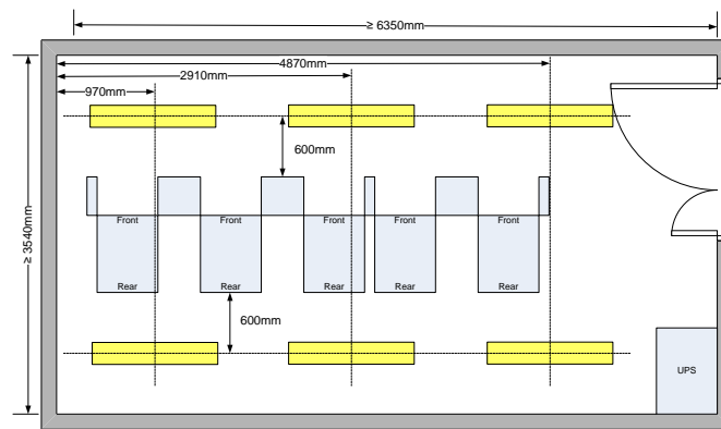
Figure 15 Lighting layout for MER A
