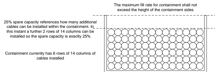
Figure 59 Example of 25% spare capacity
