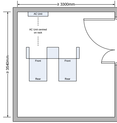
Figure 23 DX layout for MER B and SERs
