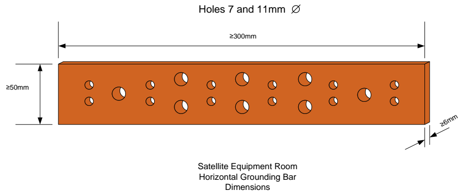
Figure 34 SER grounding bar
