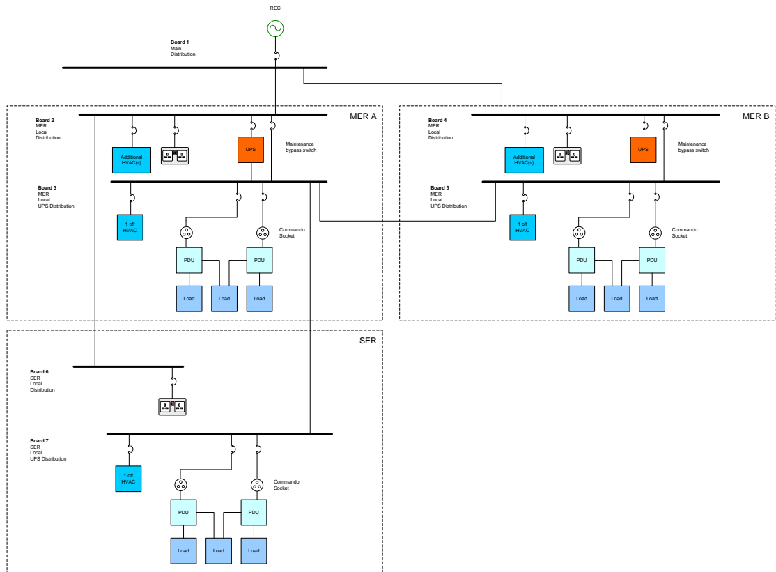
Figure 25 Telecom room power arrangements
