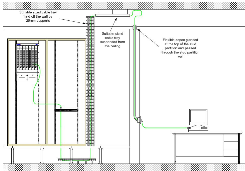
Figure 50 Stud partition outlets
