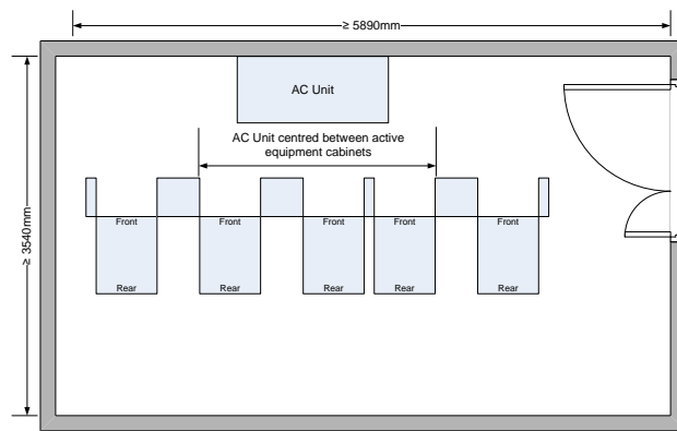
Figure 24 DX layout for MER A with UPS
