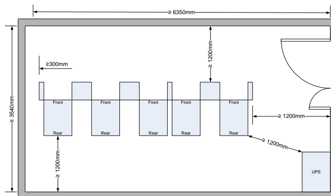
Figure 5 Telecom room layout for MER A with UPS
