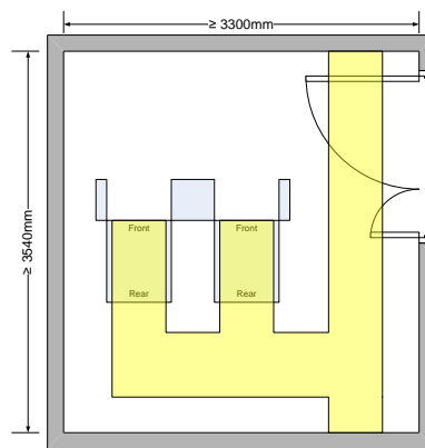
Figure 30 Suspended floor containment for MER B and SERs
