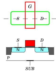
NMOS Enhancement transistor NMOS Process
