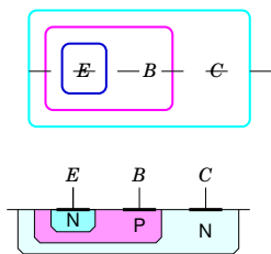
NPN Transistor
