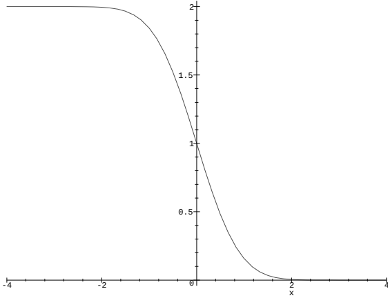
Figure 14: The complementary error function \operatorname{erfc}(x) .
