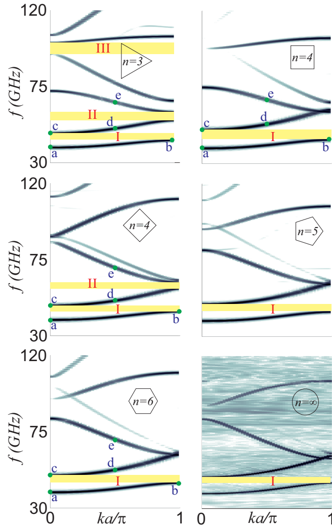
FIG. 2: (Colour Online) SW dispersion results of MAW structures marked with their respective antidot shapes as insets. Indexed band gaps are highlighted with horizontal bars.
