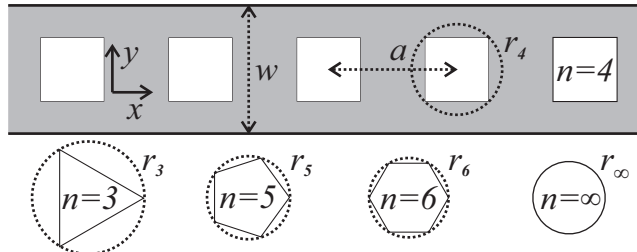
FIG. 1: (Top panel) A part of the 1D MAW structure showing square antidots (white holes in grey magnetic region) disposed along the central axis of the waveguide of width, w = 24 nm and lattice constant, a = 24 nm. The square antidots are inscribed within a circle of radius, r_4 . (Bottom panel) Other examined antidot shapes inscribed within their respective imaginary circumcircles. For n \in \{3, 4, 5, 6, \infty\} , r_n is given by Eqn. 1, where filling fraction f = 0.25 and unit cell area A = wa .
