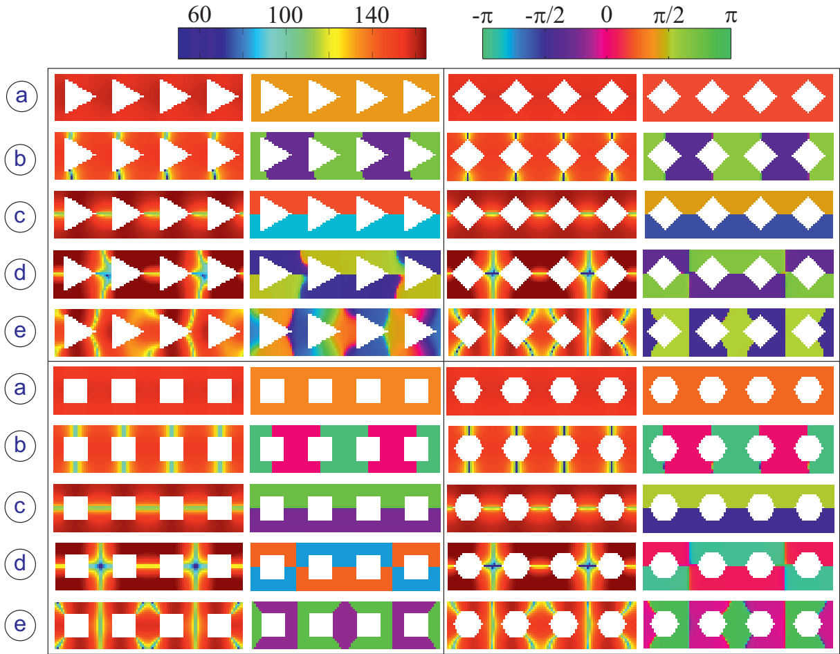
FIG. 3: (Colour Online) Power (first and third column) and phase (second and fourth column) distribution profiles corresponding to marked (k, f) locations (@ to @) in Fig. 2 for MAWs with triangular, diamond, square and hexagonal shaped antidots. Power is presented on an arbitrary logarithmic colour map while the phase profile representations use a cyclic colour map.
