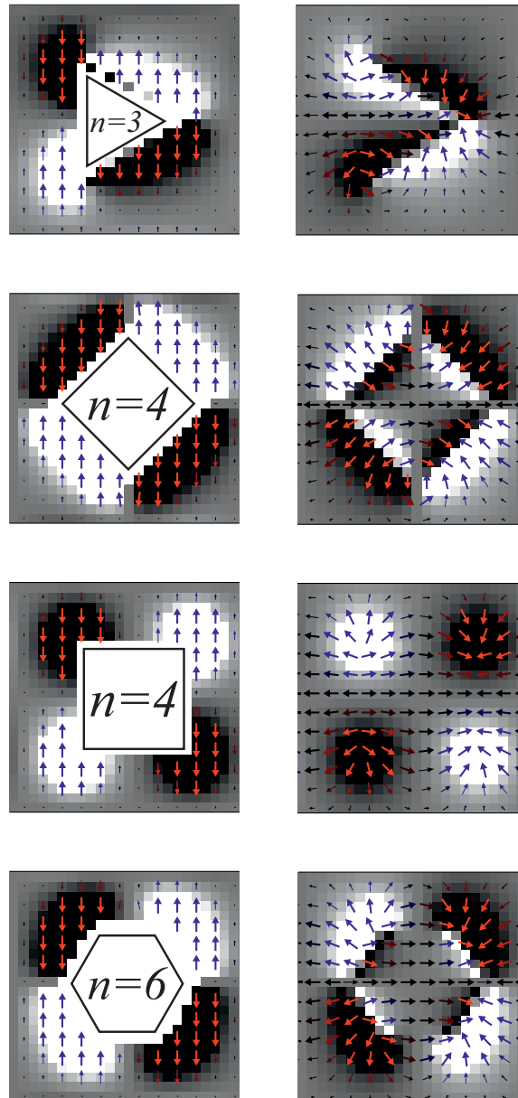
FIG. 4: (Colour Online) Exchange (left column) and demagnetization (right column) field profiles at t = 0 for n = 3, 4 & 6 (marked by insets).
