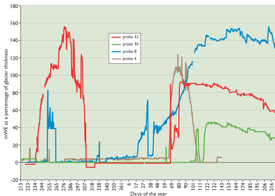
Fig. 5. Water pressure data obtained from the Glacswab wireless probes: 2004–2005 englacial probe 4 and subglacial probe 8; 2005–2006, subglacial probes 10 and 12.
