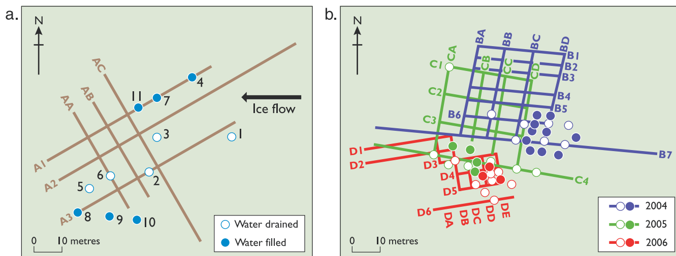
Fig. 3. (a) GPR grids 2003 (Site A); (b) GPR grids 2004, 2005 and 2006 (Site B) with boreholes shown. Open circles, water-drained holes; filled circles, water-filled boreholes. Ice flow from right to left; location on the glacier is shown in Figure 1e.
