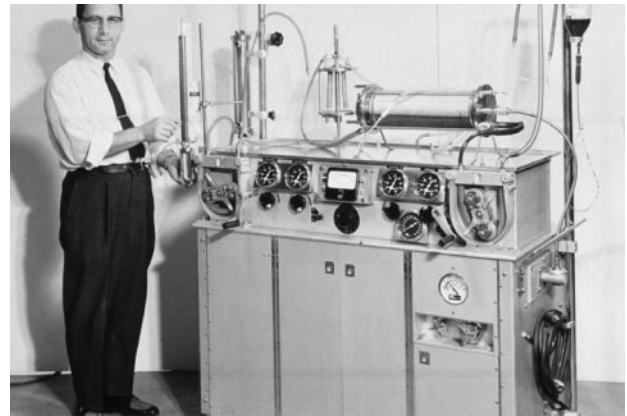
Figure 12. The Kay-Cross rotating disc heart-lung machine manufactured by Pemco Inc. Standing by the machine is William Koteles, founder of Pemco. Used with permission from Pemco Inc.
