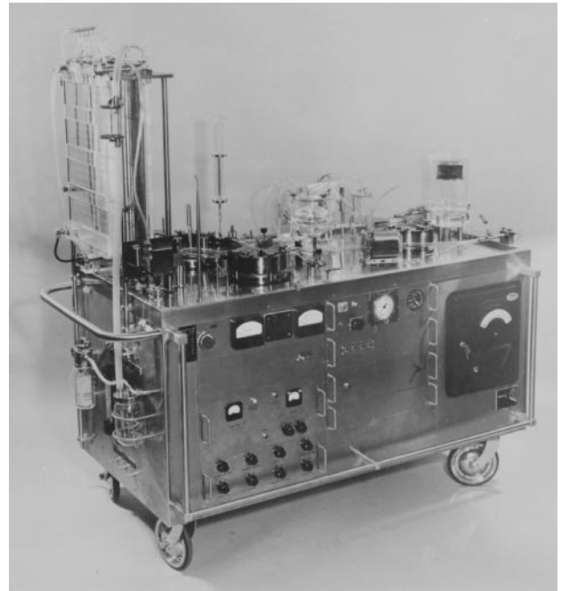
Figure 11. The Mayo-Gibbon heart-lung machine. Used with permission from the Mayo Historical Unit, Mayo Clinic, Rochester, Minn.
