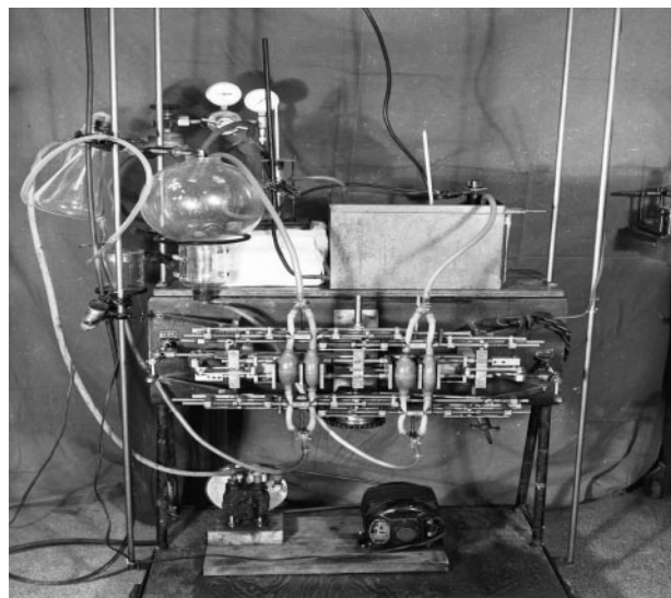
Figure 3. Heart-lung machine developed by C.R. Cowan and William Mustard. Rhesus monkey lungs were suspended in the glass flask and used as the oxygenator. Used with permission from the Hospital Library and Archives, Hospital for Sick Children, Toronto, Ontario, Canada.
