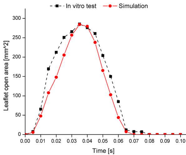
FIGURE 7. Leaflet open areas of the in vitro test and the FSI simulation during the period of 0.1 s.
