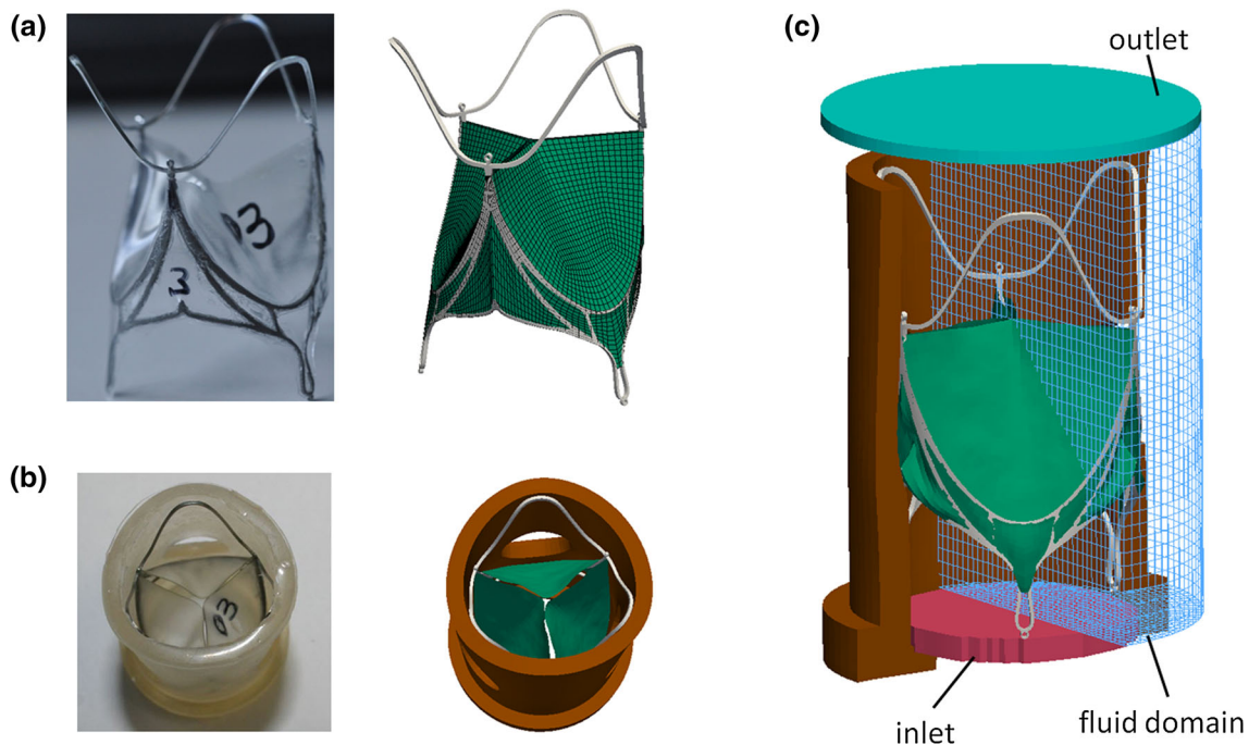
FIGURE 1. In vitro test setup and FSI models. (a) Stented valve and corresponding model where the leaflet mesh is visible. (b) The valve inserted in a silicon compartment representing the aortic root and the corresponding model. (c) FSI model including the valve, the compartment and the fluid domain; inlet and outlet sections are visible where the boundary conditions are applied in terms of pressures.
