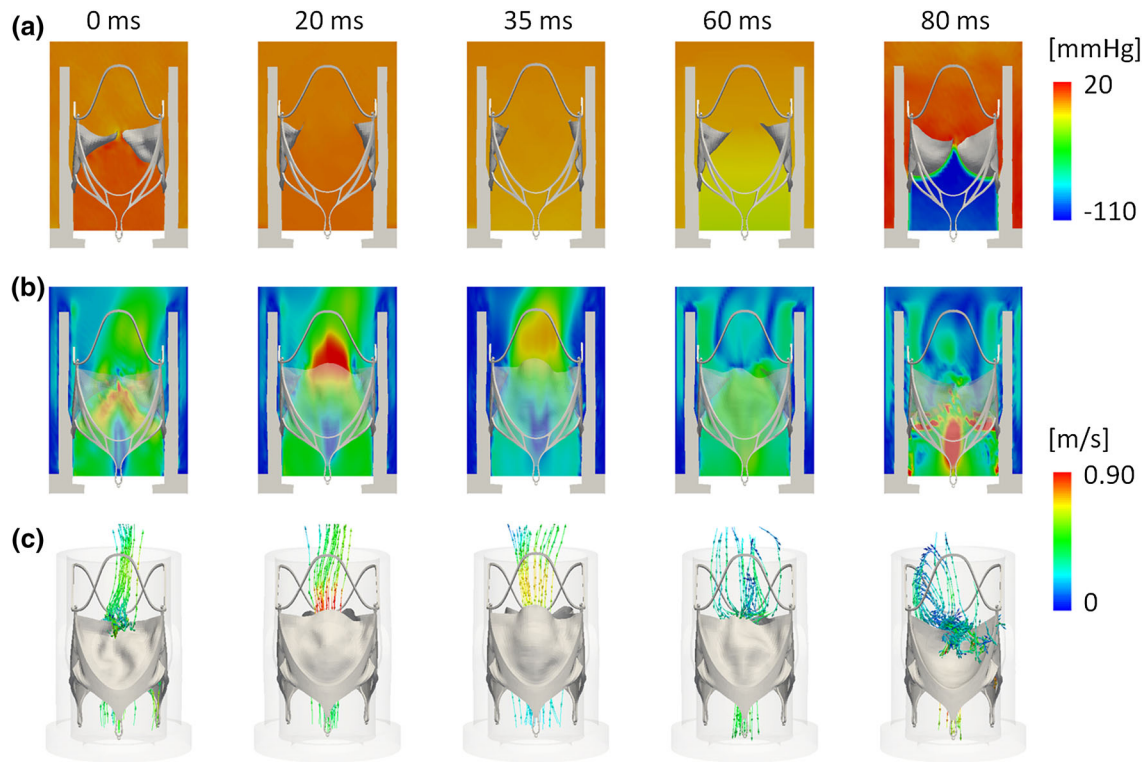
FIGURE 8. Pressure (a) and velocity (b) contour maps of the in vitro FSI simulation. Pathlines colored with respect to velocities are also reported (c).
