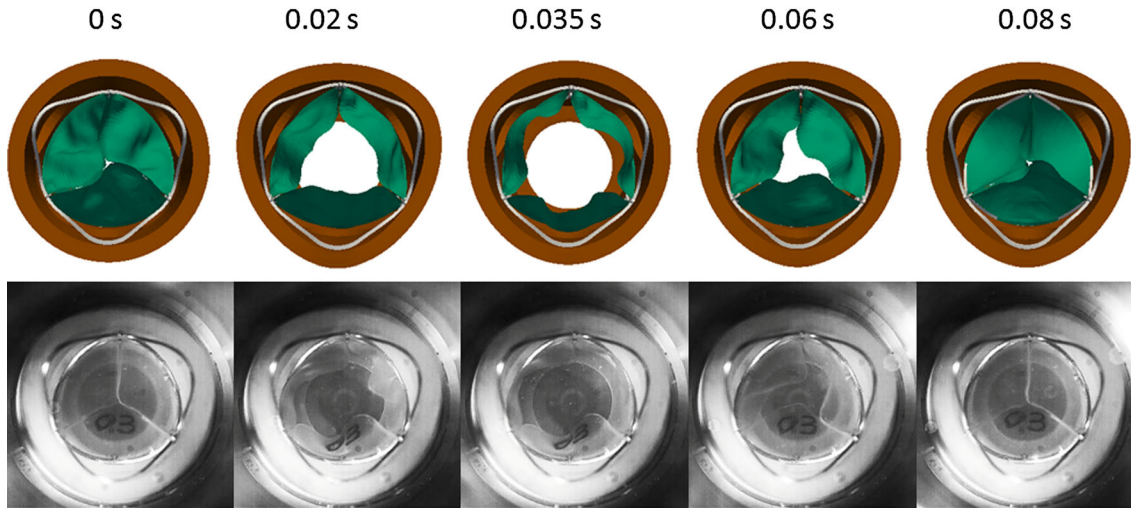
FIGURE 6. Top views of the valve kinematics at five time instances for the FSI simulation (top) and the in vitro test (bottom). The leaflet thickness in the simulation was not displayed for a better visualization.
