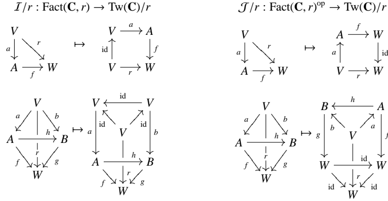
Fig. 4. I/r and J/r on objects and arrows.
