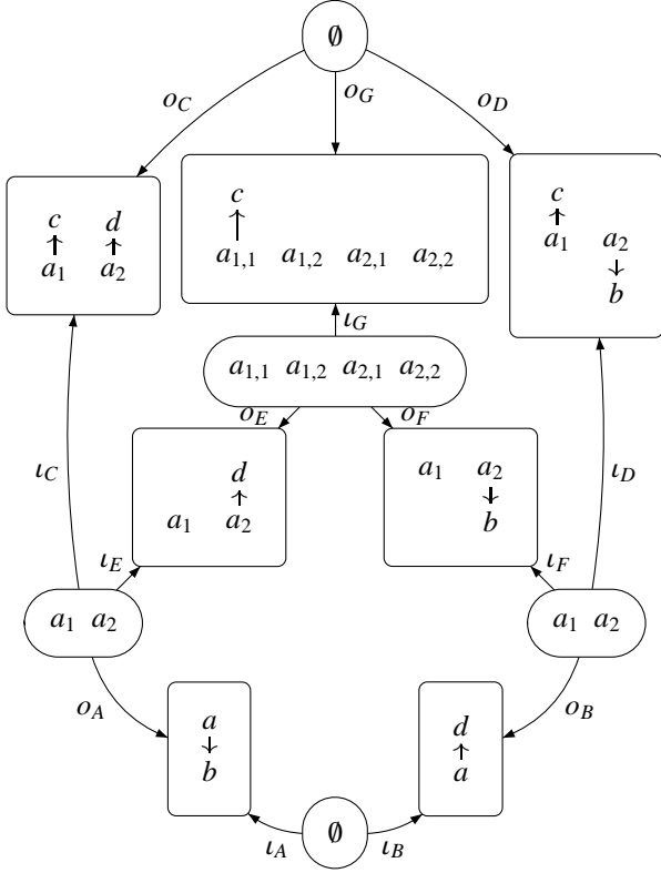
Figure 5. GRPO ILC(Graph)
