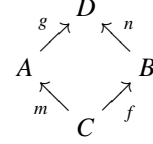
Figure 2. Pushout diagram.
