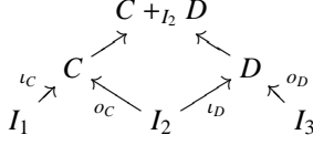
Figure 3. Composition of cospans.
