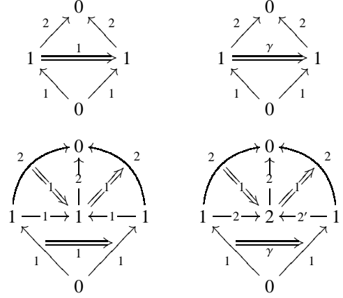
Figure 4. GRPOs in \text{ILC}(\text{Set}) .
