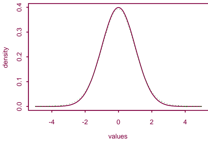
Std normal and t density with 15 df
