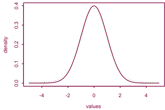
Std normal and t density with 30 df
