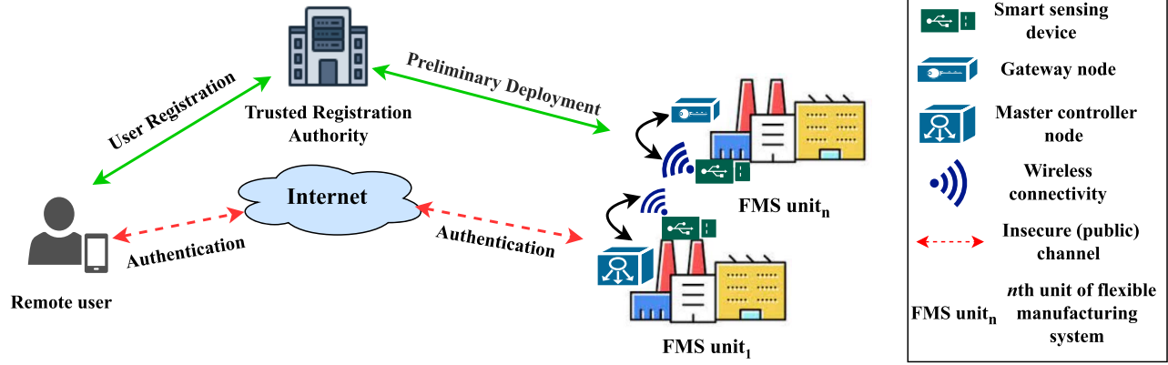
Fig. 1. Network model of flexible manufacturing monitoring system.
