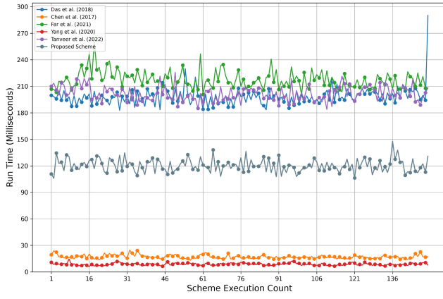
Fig. 3. Comparison of scheme runtime.
