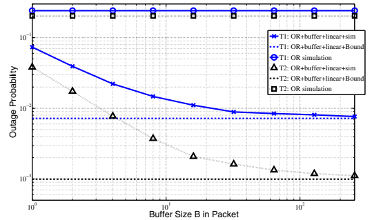
Fig. 4. The simulated and theoretical outage probability evaluated from (11).
