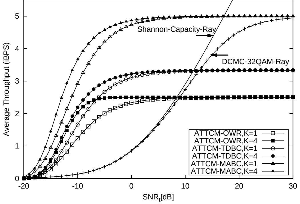
Fig. 9. iBPS versus \text{SNR}_t of the ATTCM aided one-way relay system and two-way relay system when communicating over quasi-static Rayleigh fading channels. The “DCMC-32QAM-Ray” refers to the DCMC capacity for 32QAM modulation in Rayleigh channel and the “Shannon-Capacity-Ray” refers to the CCMC capacity in Rayleigh channel. The “OWR” is represented by one-way relay system. A BER below 10^{-5} is maintained and G_{sr} = G_{rd} = 8 .
