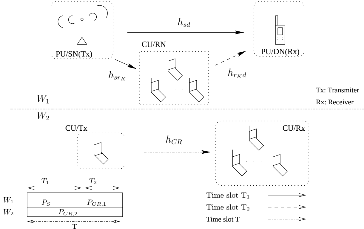
Fig. 1. The PU's and CU's spectrum-access model. The bandwidth, time period and power allocation for the PU and CU. The total time slot duration is T = T_1 + T_2 and the bandwidth is W_0 = W_1 + W_2
