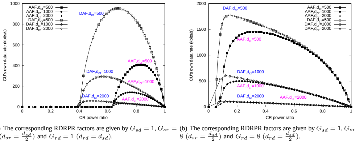
Fig. 6. The CU's own data rate based on DAF and AAF detections.
