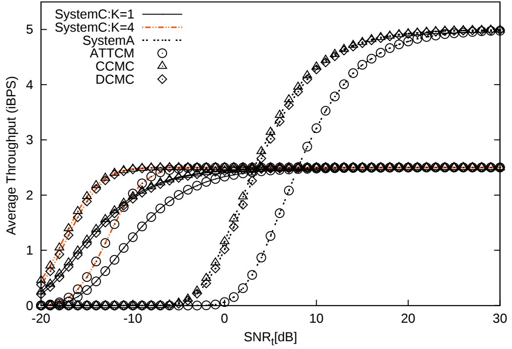
Fig. 7. iBPS versus \text{SNR}_t of the ATTTCM, CCMC and DCMC aided CR schemes when communicating over quasi-static Rayleigh fading channels. A BER below 10^{-5} is maintained and G_{sr} = G_{rd} = 8 . The “SystemC” is represented by relay aided system of Section II-C.2, while the “SystemA” is refer to the non-cooperative System A of Section II-C.2. The number of relays is K = 1 and K = 4 .
