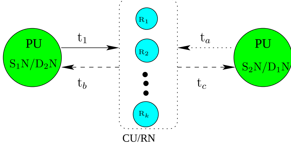
Fig. 4. The schematic of a two-way relay-aided system, including two PUs and K CUs. For MABC, t_a = t_1 and t_b = t_c = t_2 , where t_1 is the first transmission period and t_2 is the second transmission period. For TDBC, t_a = t_2 and t_b = t_c = t_3 , where t_3 is the third transmission period.
