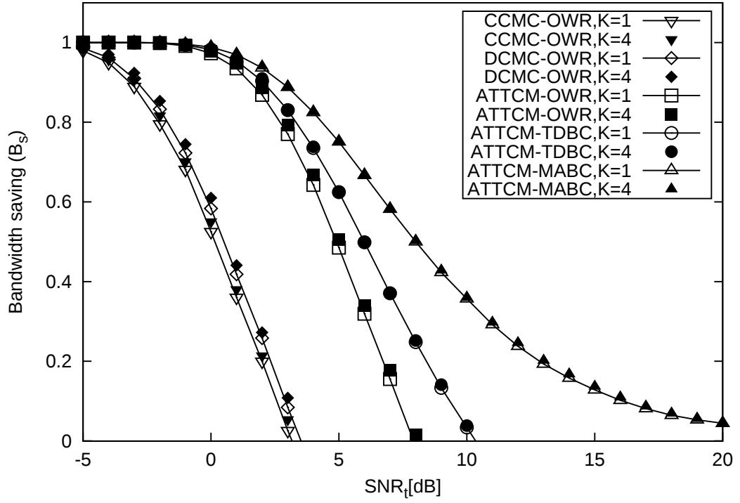
Fig. 10. Bandwidth reduction B_s versus \text{SNR}_t for ATTCM aided one-way relay and two-way relay CR schemes, when communicating over flat Rayleigh fading channels and maintaining a BER below 10^{-5} . The number of frames simulated was 1000. The “OWR” is represented by one-way relay system. G_{sr} = G_{rd} = 8 , The number of RNs in these schemes is K = 1 and K = 4 .
