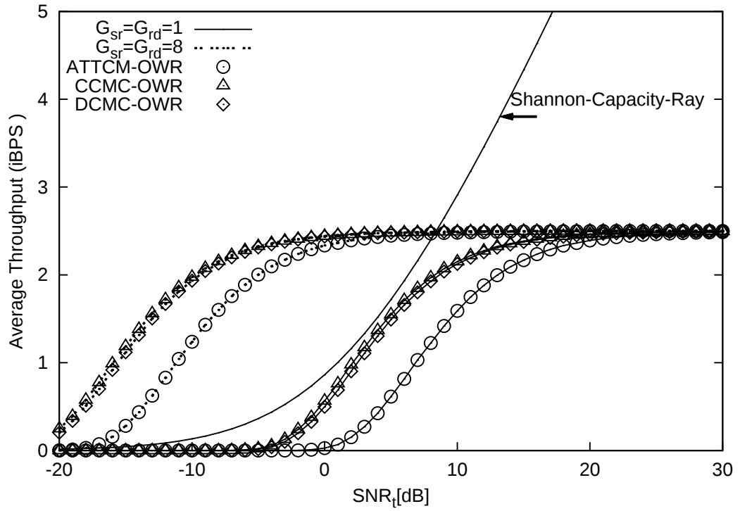
Fig. 8. iBPS versus \text{SNR}_t of the ATTTCM, CCMC and DCMC aided one-way relay in CR schemes when communicating over quasi-static Rayleigh fading channels compared to the CCMC capacity in Rayleigh channel. The “Shannon-Capacity-Ray” label refers to the CCMC capacity in Rayleigh channel. The number of relays is K = 1 . The “OWR” is represented by one-way relay system. The corresponding RDRPR are G_{sr} = G_{rd} = 8 and G_{sr} = G_{rd} = 1 .
