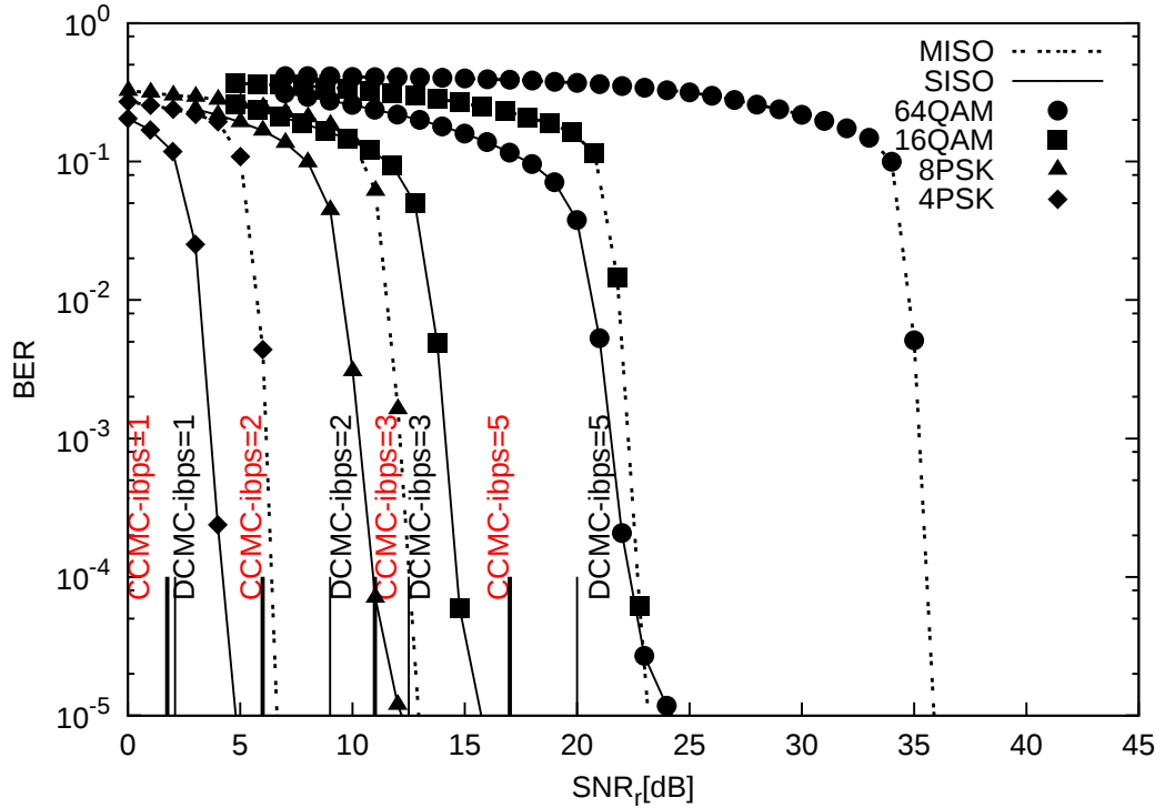
Fig. 3. The BER versus \text{SNR}_r performance of TTCM aided MISO system and TTCM aided SISO system. A frame length of 1200 symbols was employed when communicating over uncorrected Rayleigh channels. Four TTCM iterations and four outer iterations with the MISO detector is used in MISO system.
