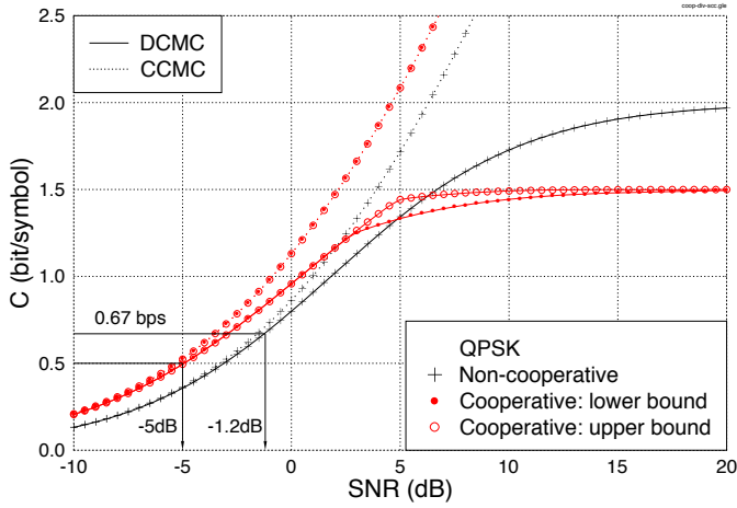
Fig. 24. The DCMC and CCMC capacity curves of cooperative network and non-cooperative QPSK assisted schemes. It can be seen that the DCMC of a cooperative network is -5 dB at 0.5 bps. DCMC of a non-cooperative QPSK assisted scheme is -1.20 dB at 0.67 bps.
