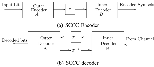
Fig. 2. The schematic of an SCCC encoder and decoder.
